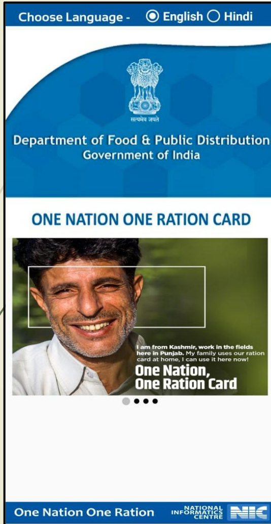
SPLASH SCREEN
